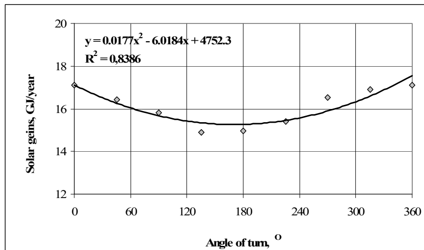
Fig. 11. The influence of location of the building in relation to the directions of the world on solar gains (own research)
